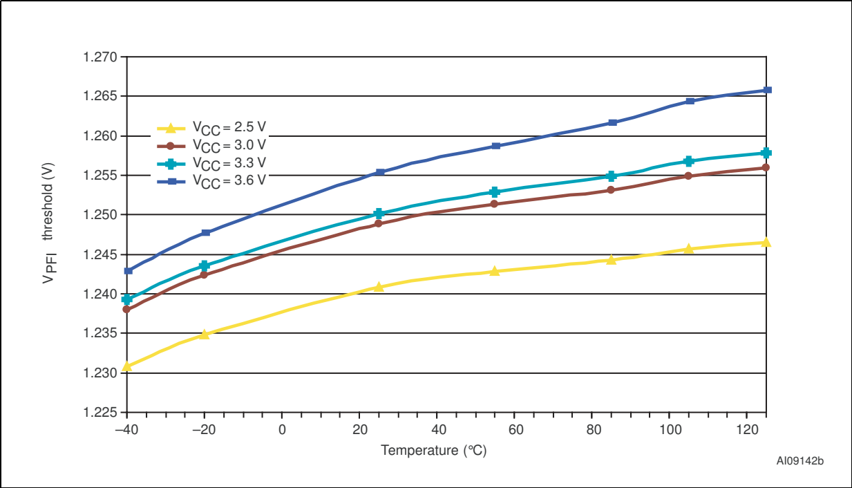
Figure 19. V_{PF1} threshold vs. temperature
