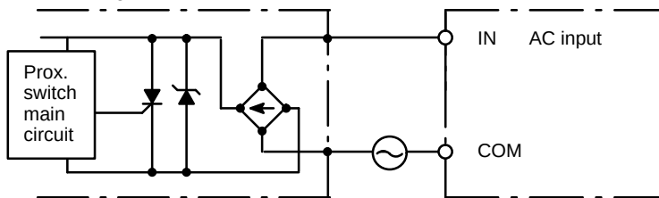
AC Switching
