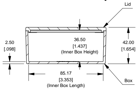
SECTION B-B Side View of Assembly
