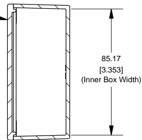
SECTION A-A End View of Assembly
