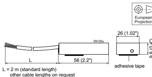
Fig. 49 Battery temperature sensor
