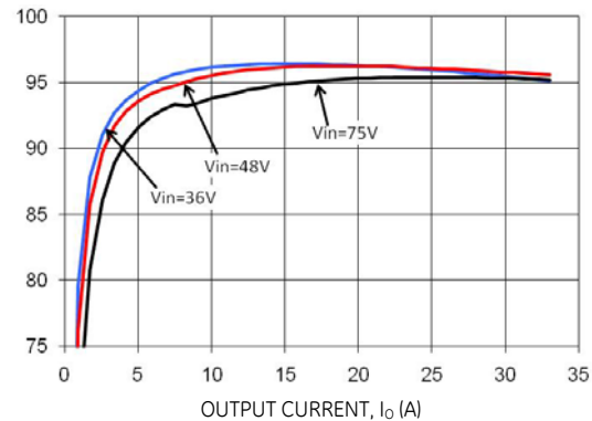
Figure 2. Typical Converter Efficiency vs. Output Current.
