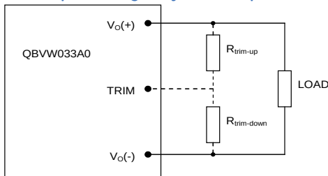
Figure 16. Circuit Configuration to Trim Output Voltage.
