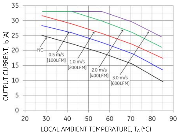
Figure 19. Output Current Derating for the Open Frame QBW033A0B in the Transverse Orientation; Airflow Direction from Vin(-) to Vin(+); Vin = 48V.
