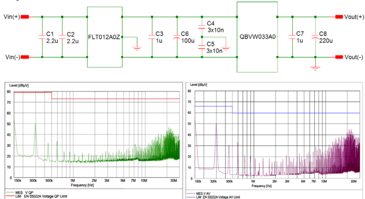
Figure 26. EMC Considerations
