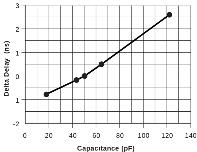
Figure 34: Delay Factor at Various Capacitive Loads
