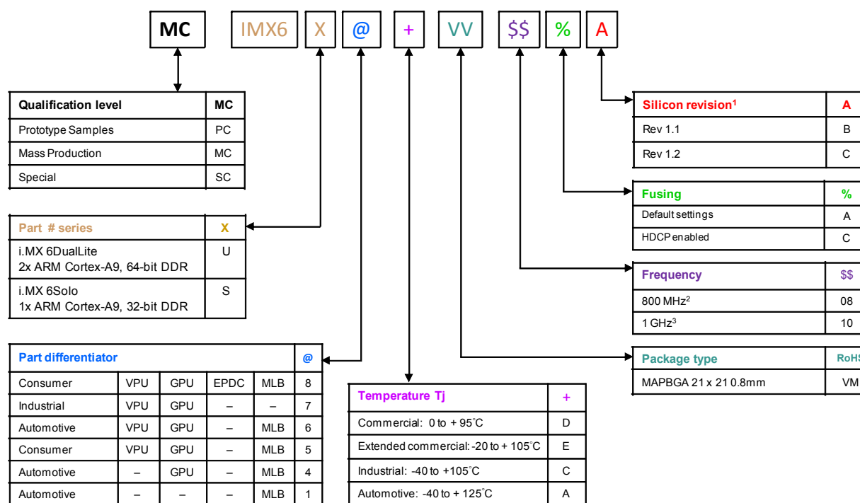
Figure 1. Part Number Nomenclature—i.MX 6Solo and 6DualLite
