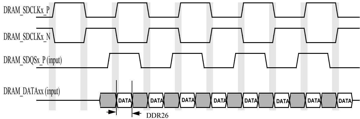
Figure 26. DDR3/DDR3L Read Cycle
