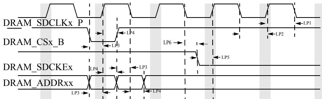
Figure 27. LPDDR2 Command and Address Timing Parameters
