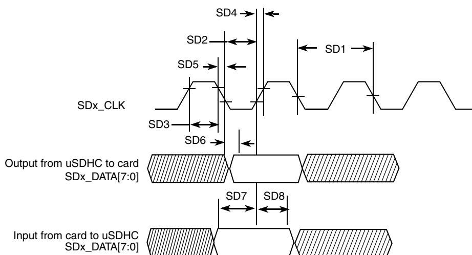
Figure 45. SD/eMMC4.3 Timing
