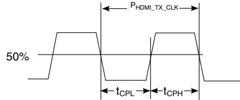
Figure 59. TMD5 Clock Signal Definitions
