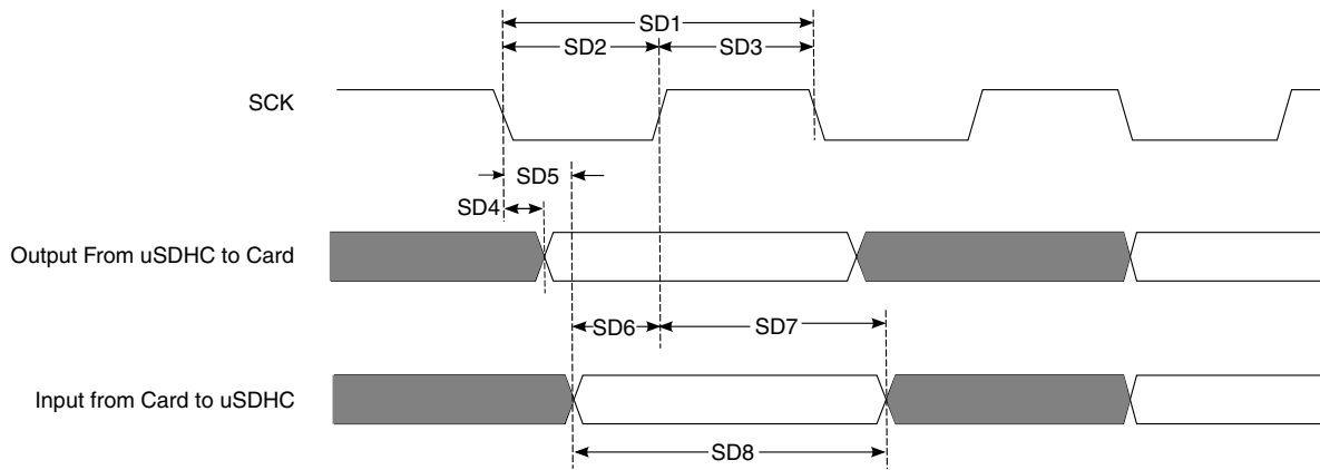
Figure 47. SDR50/SDR104 Timing
