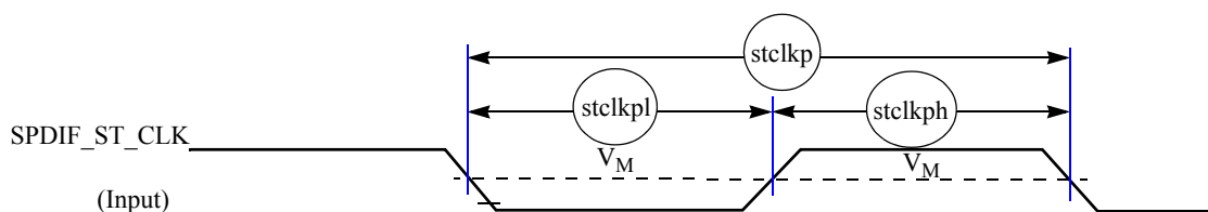
Figure 95. SPDIF_ST_CLK Timing Diagram
