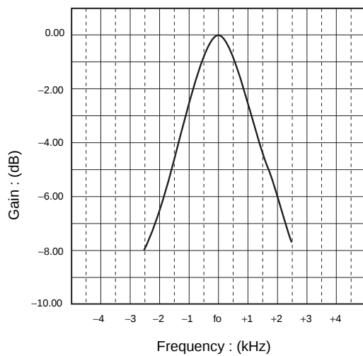
Fig.6 RPM7157 Series BPF Characteristics
