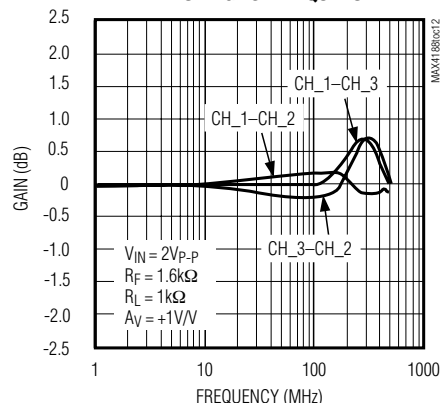
MAX4189 SMALL-SIGNAL GAIN MATCHING vs. FREQUENCY
