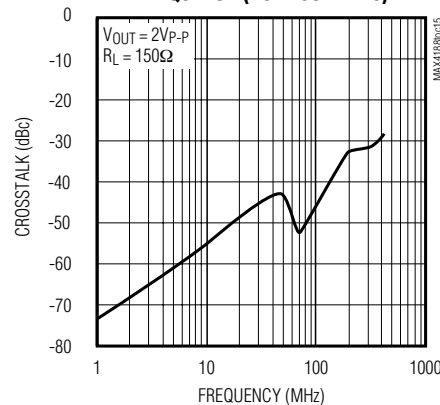
MAX4188 CROSSTALK vs. FREQUENCY (DUAL SUPPLIES)
