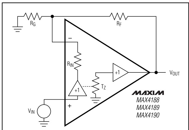
Figure 2. Current-Feedback Amplifier
