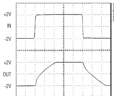
MAX4189 LARGE-SIGNAL PULSE RESPONSE
