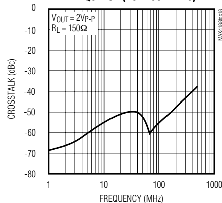
MAX4189 CROSSTALK vs. FREQUENCY (DUAL SUPPLIES)
