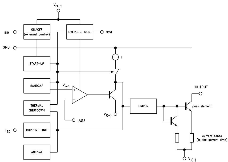
Figure 1. Block diagram
