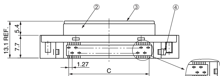
For 68 or 100-contact connector
