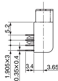
Recommended PCB layout (Connector side) t = 1.6 mm
