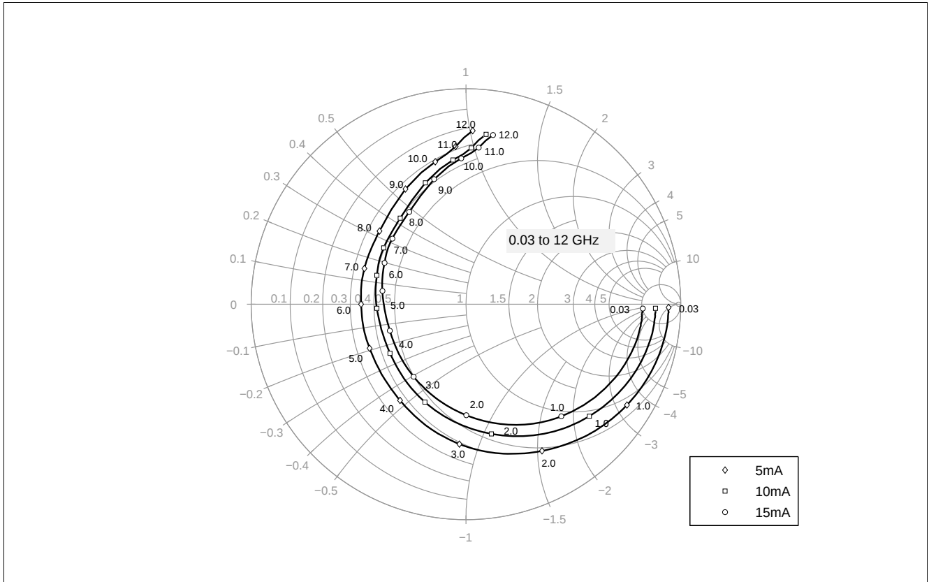
Figure 5-15 Input Reflection Coefficient S_{11} = f(f) , V_{CE} = 1.8 V, I_C = 5 / 10 / 15 mA
