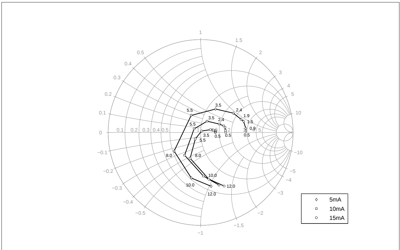
Figure 5-16 Source Impedance for Minimum Noise Figure Z_{opt} = f(f) , V_{CE} = 1.8 V, I_C = 5 / 10 / 15 mA
