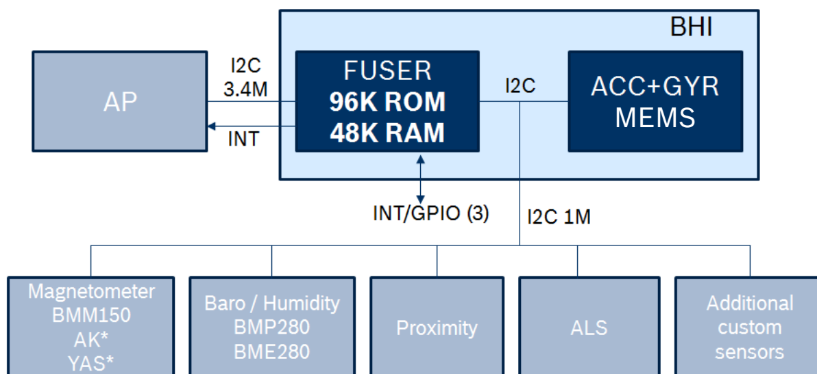
Figure 3: Block Diagram
