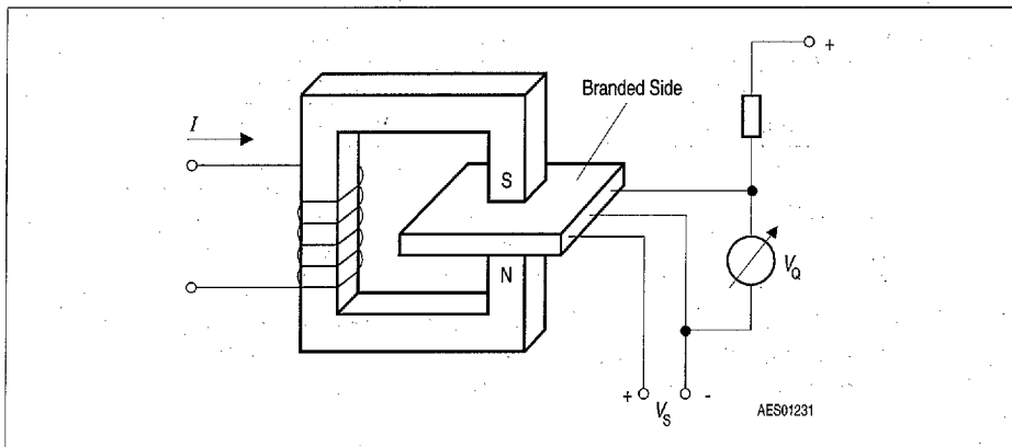
Figure 5 Sensor/Magnetic-Field Configuration
