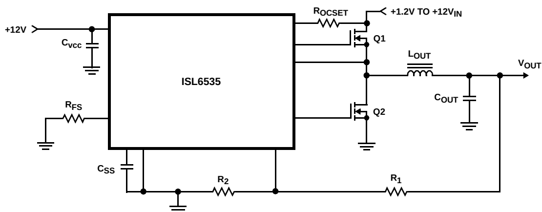
FIGURE 2. SIMPLIFIED POWER SYSTEM DIAGRAM
