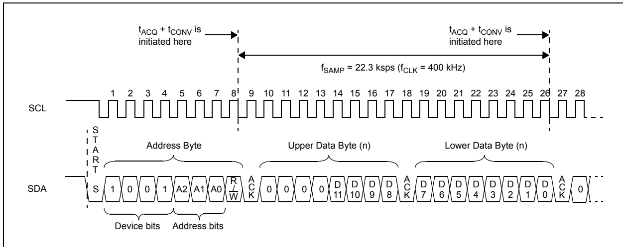
FIGURE 5-6: Continuous Conversion.
