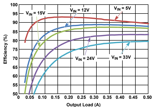
Figure 9. Efficiency vs Load, PWM, V_{OUT} = 3.3\text{V}
