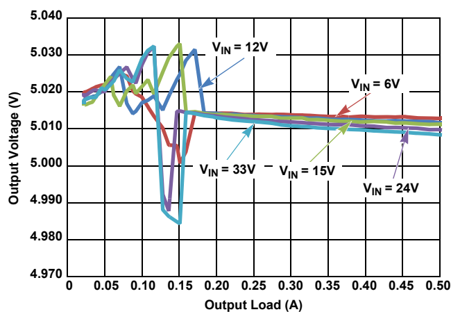
Figure 28. V_{OUT} Regulation vs Load, PFM, V_{OUT} = 5\text{V}
