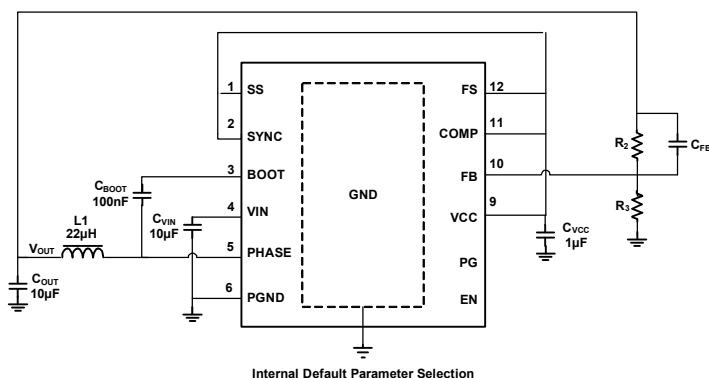
Figure 1. Typical Application
