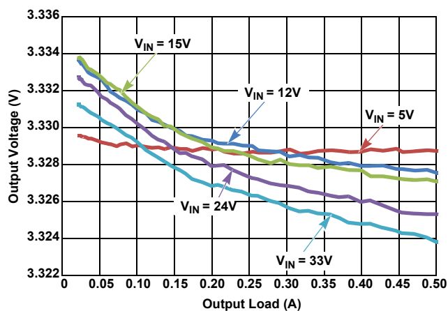
Figure 14. V_{OUT} Regulation vs Load, PWM, V_{OUT} = 3.3\text{V}
