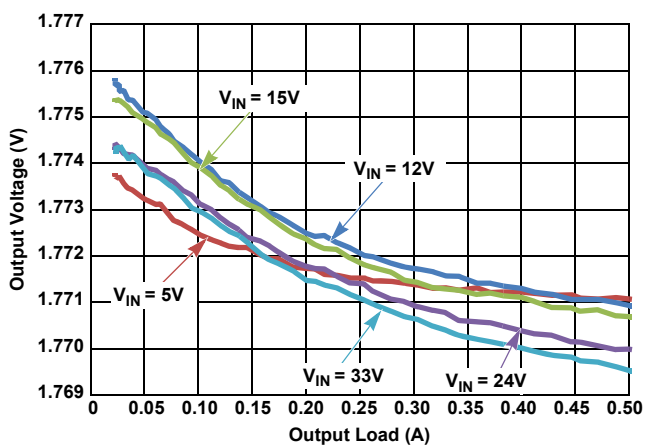
Figure 16. V_{OUT} Regulation vs Load, PWM, V_{OUT} = 1.8\text{V}
