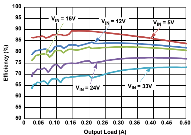
Figure 10. Efficiency vs Load, PFM, V_{OUT} = 1.8\text{V}
