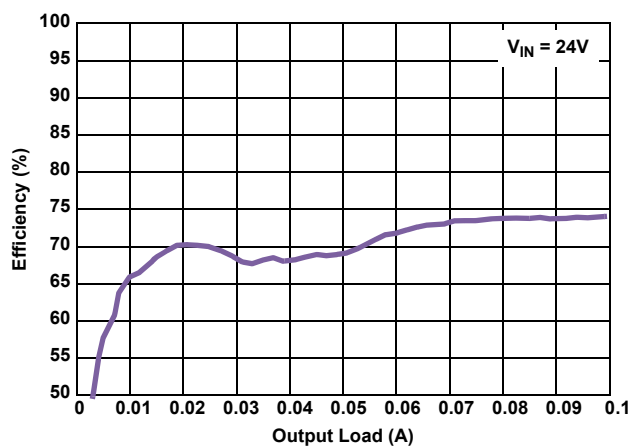
Figure 24. Efficiency vs Load, PFM, V_{OUT} = 1.8\text{V}
