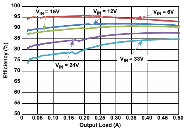
Figure 6. Efficiency vs Load, PFM, V_{OUT} = 5\text{V}
