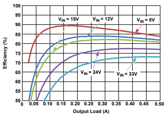
Figure 11. Efficiency vs Load, PWM, V_{OUT} = 1.8\text{V}
