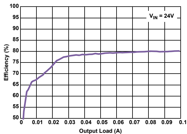
Figure 25. Efficiency vs Load, PFM, V_{OUT} = 3.3\text{V}
