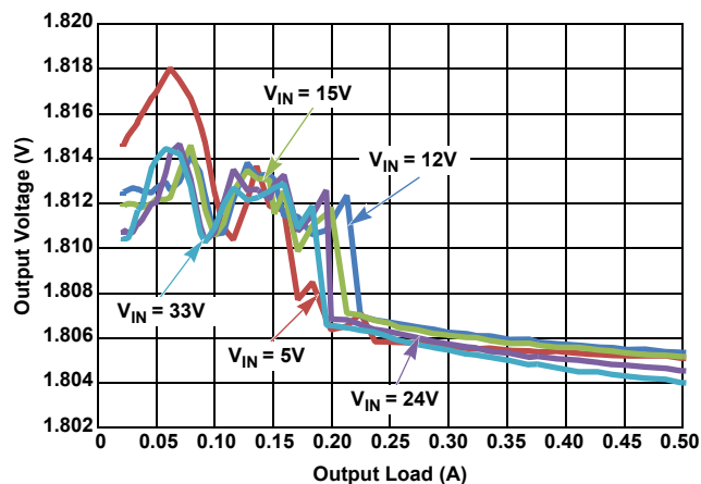
Figure 32. V_{OUT} Regulation vs Load, PFM, V_{OUT} = 1.8\text{V}
