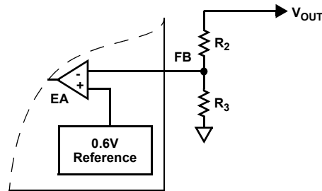
Figure 59. External Resistor Divider
