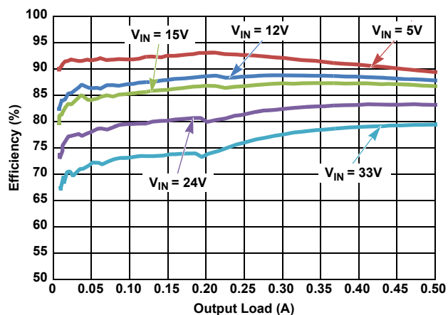
Figure 8. Efficiency vs Load, PFM, V_{OUT} = 3.3\text{V}
