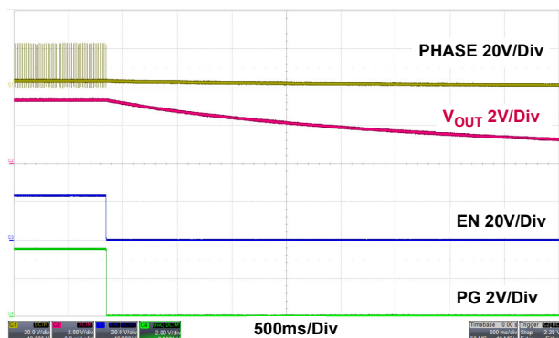
Figure 35. Shutdown at No Load, PFM
