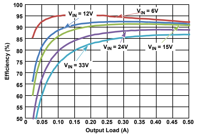
Figure 19. Efficiency vs Load, PMW, V_{OUT} = 5V
