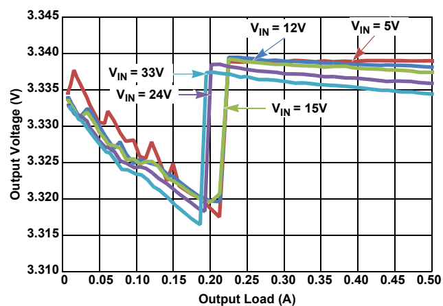
Figure 15. V_{OUT} Regulation vs Load, PFM, V_{OUT} = 3.3\text{V}
