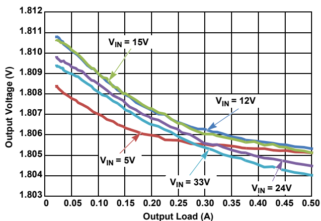
Figure 31. V_{OUT} Regulation vs Load, PWM, V_{OUT} = 1.8\text{V}
