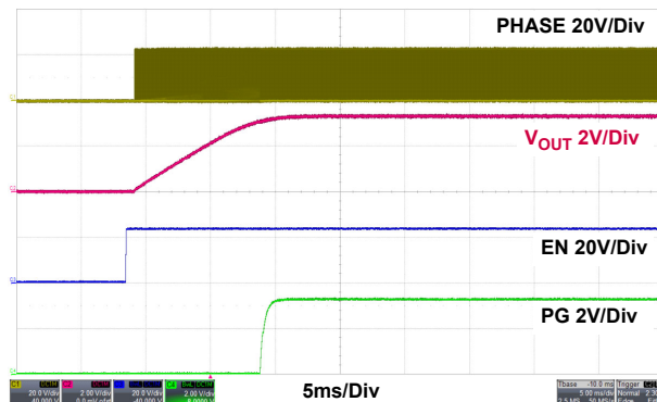
Figure 34. Start-Up at No Load, PWM
