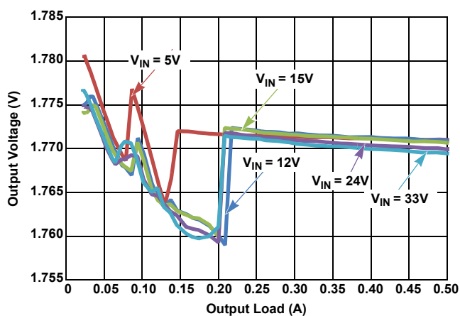
Figure 17. V_{OUT} Regulation vs Load, PFM, V_{OUT} = 1.8\text{V}
