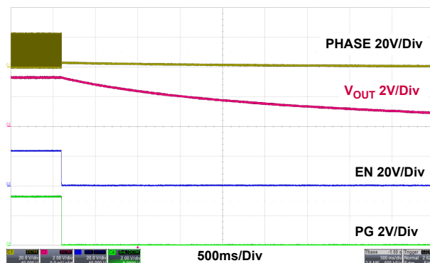
Figure 36. Shutdown at No Load, PWM
