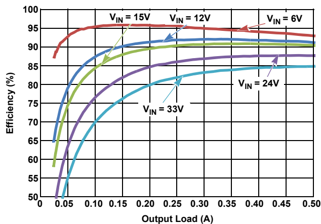
Figure 7. Efficiency vs Load, PWM, V_{OUT} = 5\text{V}
