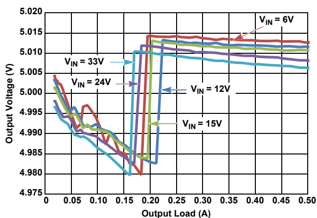
Figure 13. V_{OUT} Regulation vs Load, PFM, V_{OUT} = 5\text{V}
