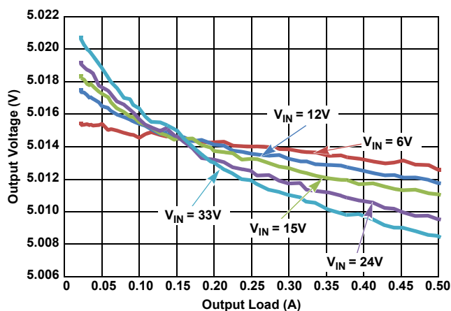
Figure 27. V_{OUT} Regulation vs Load, PWM, V_{OUT} = 5\text{V}
