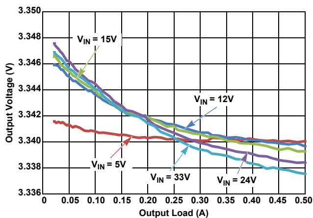
Figure 29. V_{OUT} Regulation vs Load, PWM, V_{OUT} = 3.3\text{V}
