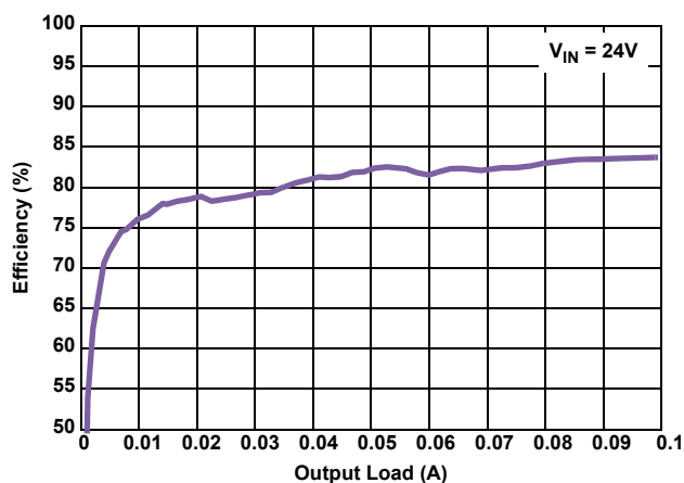
Figure 26. Efficiency vs Load, PFM, V_{OUT} = 5\text{V}
