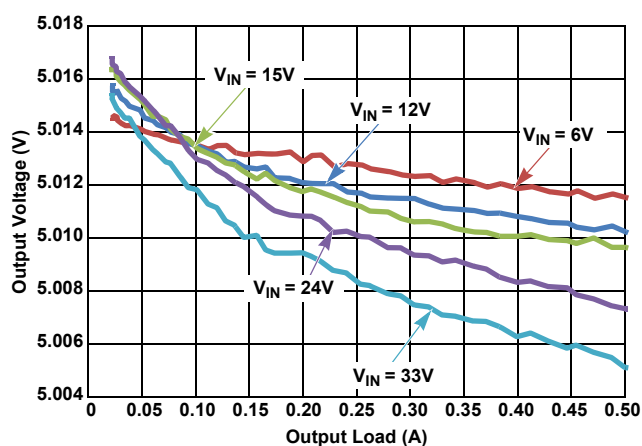
Figure 12. V_{OUT} Regulation vs Load, PWM, V_{OUT} = 5\text{V}
