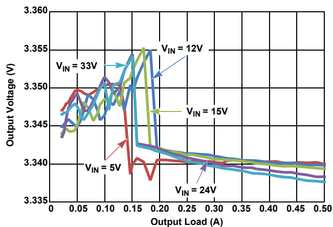
Figure 30. V_{OUT} Regulation vs Load, PFM, V_{OUT} = 3.3\text{V}
