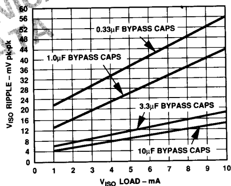
Figure 8. Isolated Power Supply Ripple (mV pk-pk) vs. Load (mA) and Bypass Capacitance ( \mu F )
