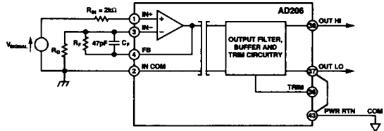
Figure 12. Noninverting Input Configuration for a Gain
