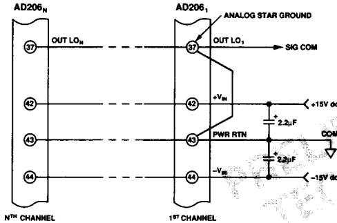
Figure 10. Powering the AD206
