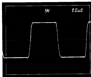
Figure 7. Output Response of the AD206 to a + and - Full-Scale Step at the Isolator's Input, with a Gain of 1 ( R_L = 2 k\Omega )
