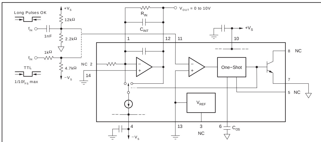
Figure 4. Frequency-to-Voltage Conversion
