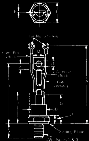
Conforms to TO-94 Outline
