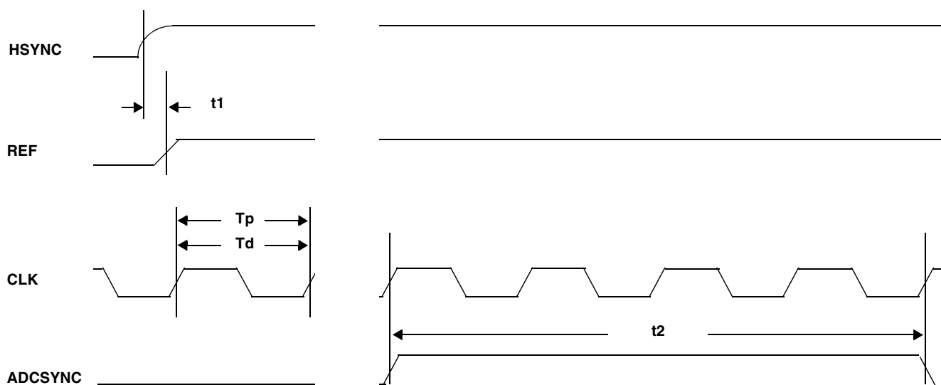
Figure 10-5. Timing for Phase-Locked Loop
