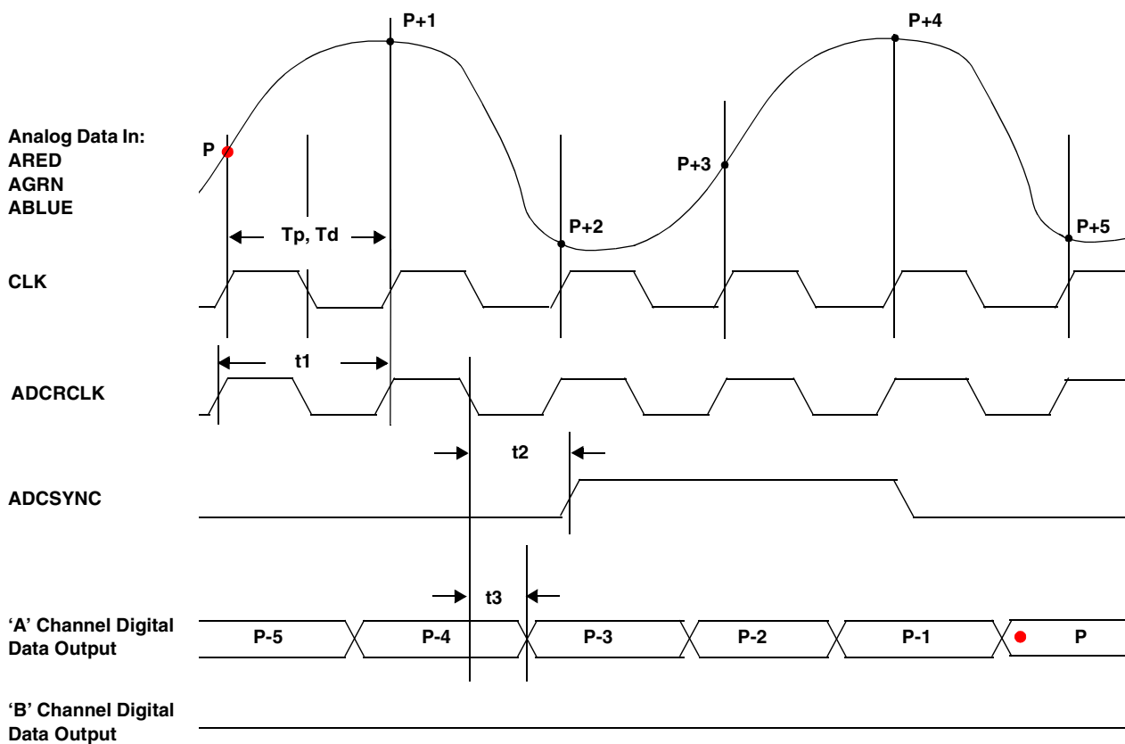
Figure 10-7. AC Timing for 1-Pixel-per-Clock Mode
