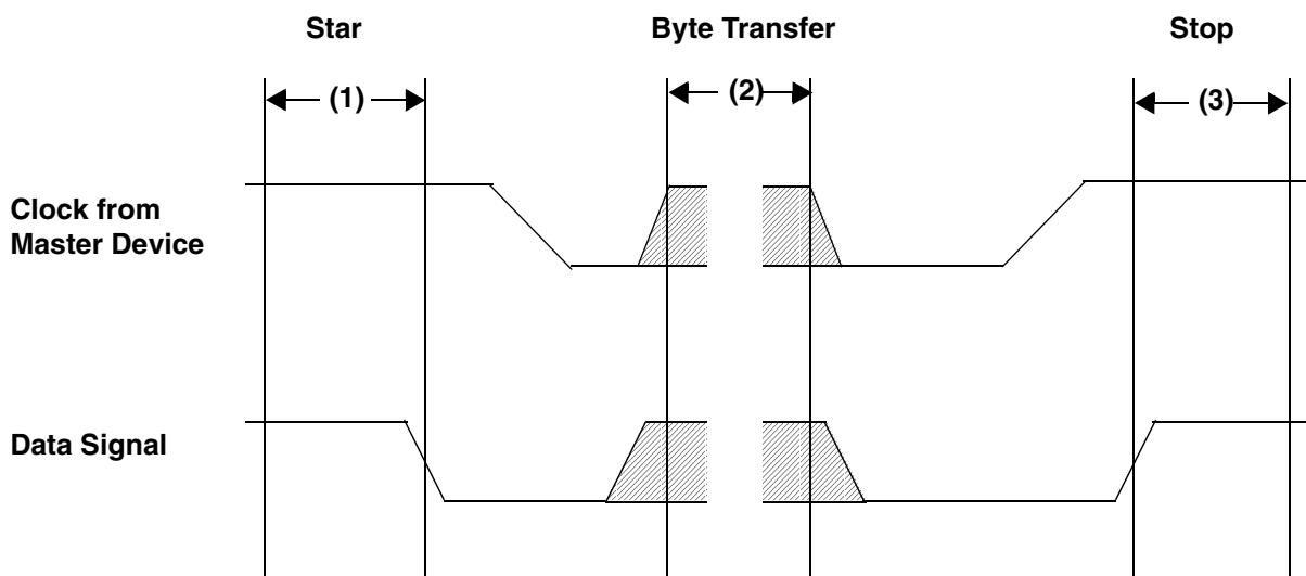
Figure 10-1. Start and Stop Conditions
