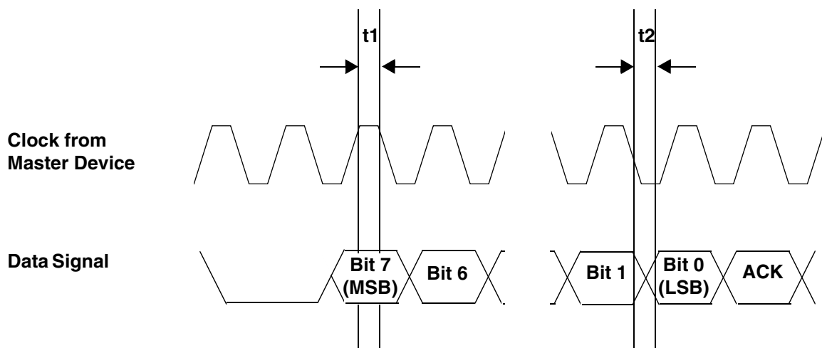
Figure 10-2. Byte Transfer on Industry-Standard 2-Wire Serial Bus
