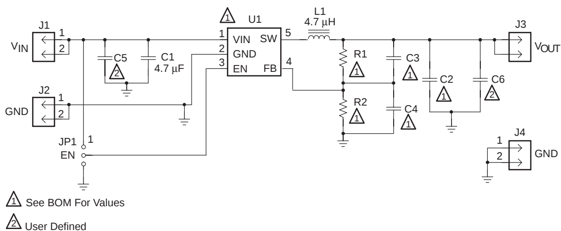
Figure 4-1. TPS6222x Schematic
