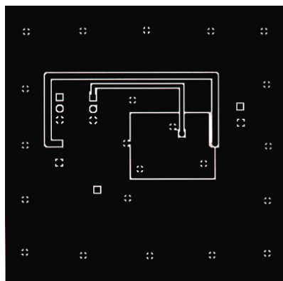
FIGURE 9. Buck—Bottom Layer
