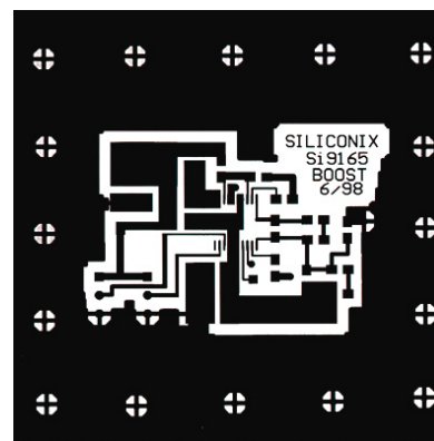
FIGURE 11. Boost—Top Layer
