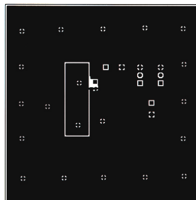
FIGURE 12. Boost—Bottom Layer
