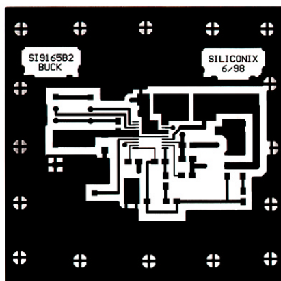
FIGURE 8. Buck—Top Layer
