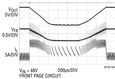
Short-Circuit/ Foldback Operation
