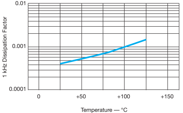
Dissipation Factor vs. Temperature Radial
