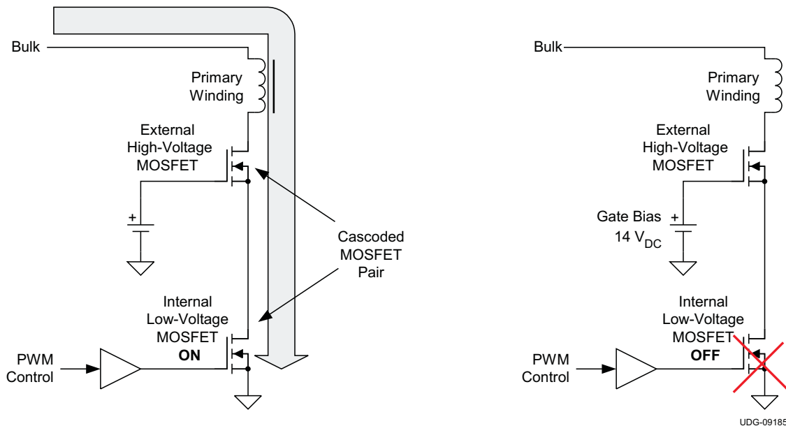
Figure 18. Cascoded Architecture
