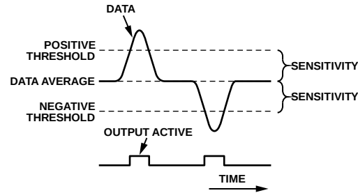
Figure 20. Threshold Sensitivity
