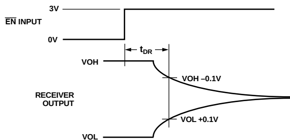
Figure 22. Receiver-Disable Timing
