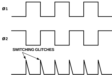
Figure 31. Switching Glitches
