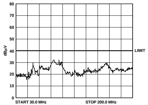
Figure 14. EMC Radiated Emissions
