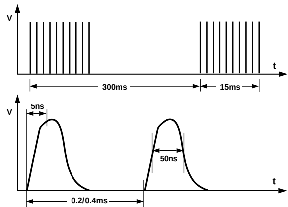
Figure 28. IEC1000-4-4 Fast Transient Waveform
