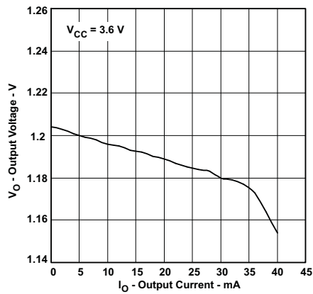
Figure 15. VDD_ALIVE Output Voltage vs Output Current
