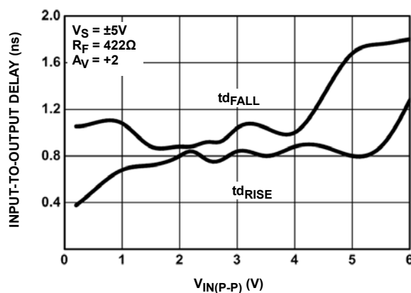
FIGURE 16. INPUT-TO-OUTPUT DELAY
