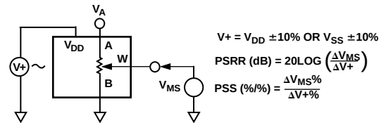
Figure 34. Power Supply Sensitivity Test Circuit (PSS, PSRR)
