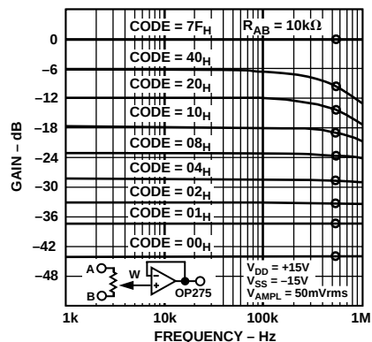
Figure 14. 10 k \Omega Gain vs. Frequency vs. Code
