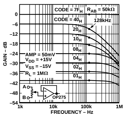
Figure 17. 50 k \Omega Gain vs. Frequency vs. Code
