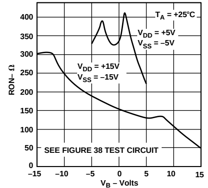
Figure 25. Incremental Wiper Contact Resistance vs. Common-Mode Voltage
