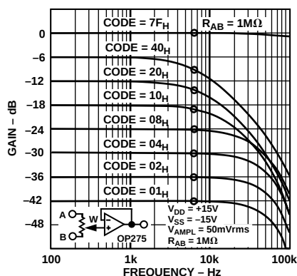
Figure 15. 1 M \Omega Gain vs. Frequency vs. Code
