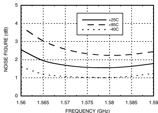
Noise Figure vs. Temperature [4]
