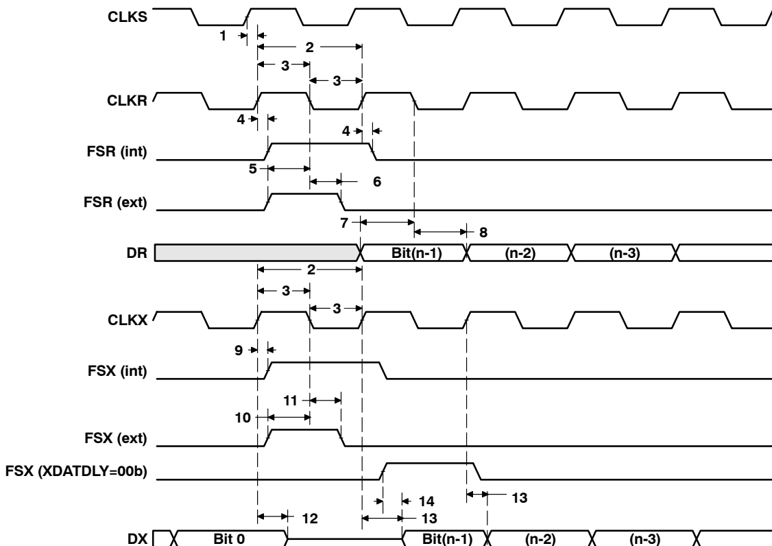
Figure 50. McBSP Timings
