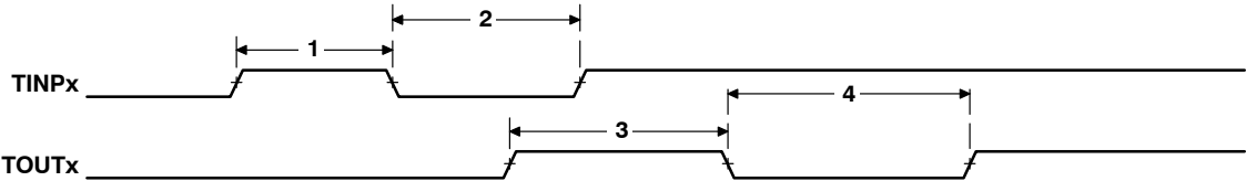
Figure 57. Timer Timing
