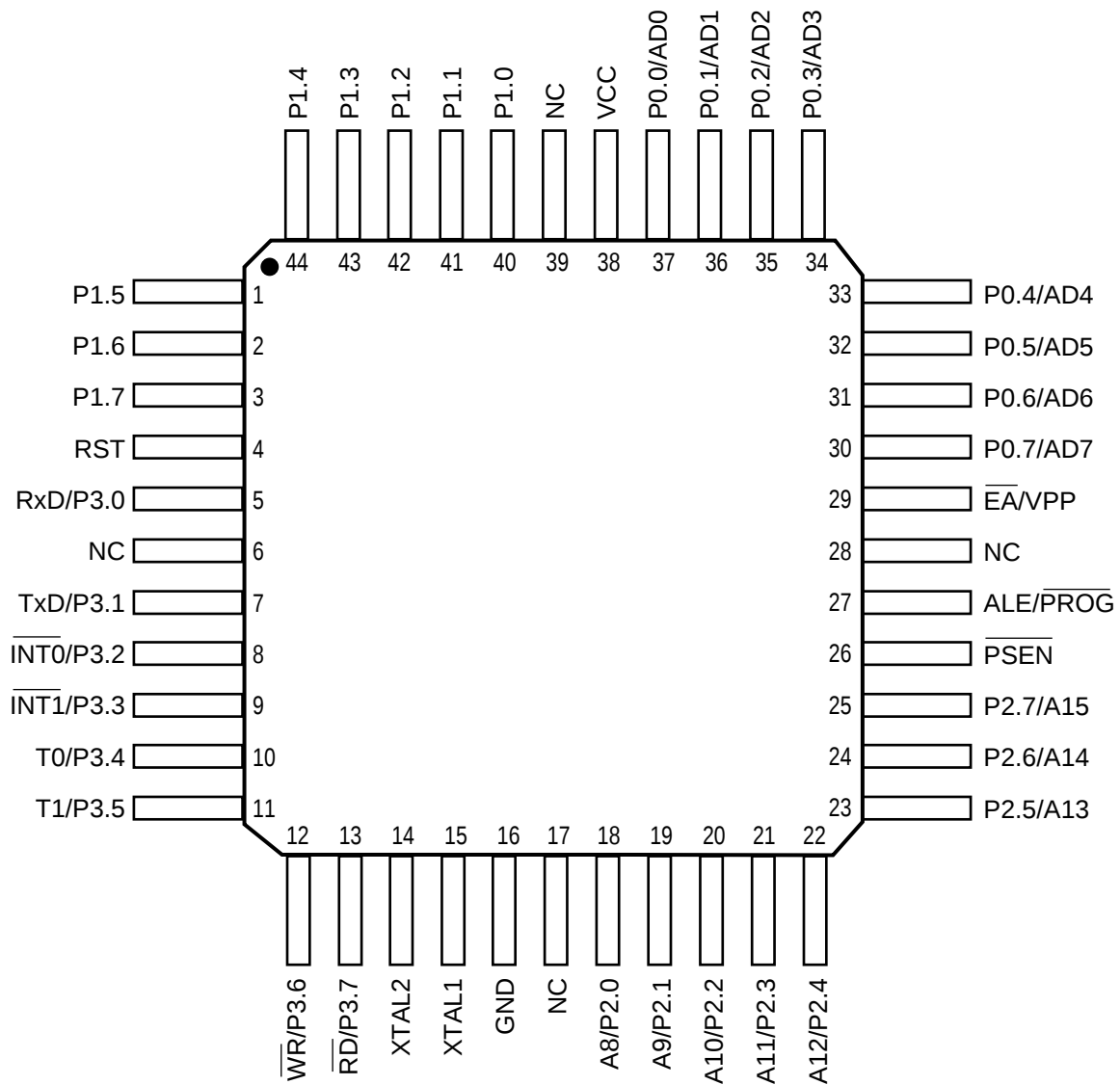
Figure 3. IS80C51/31 Pin Configuration: 44-pin PQFP
