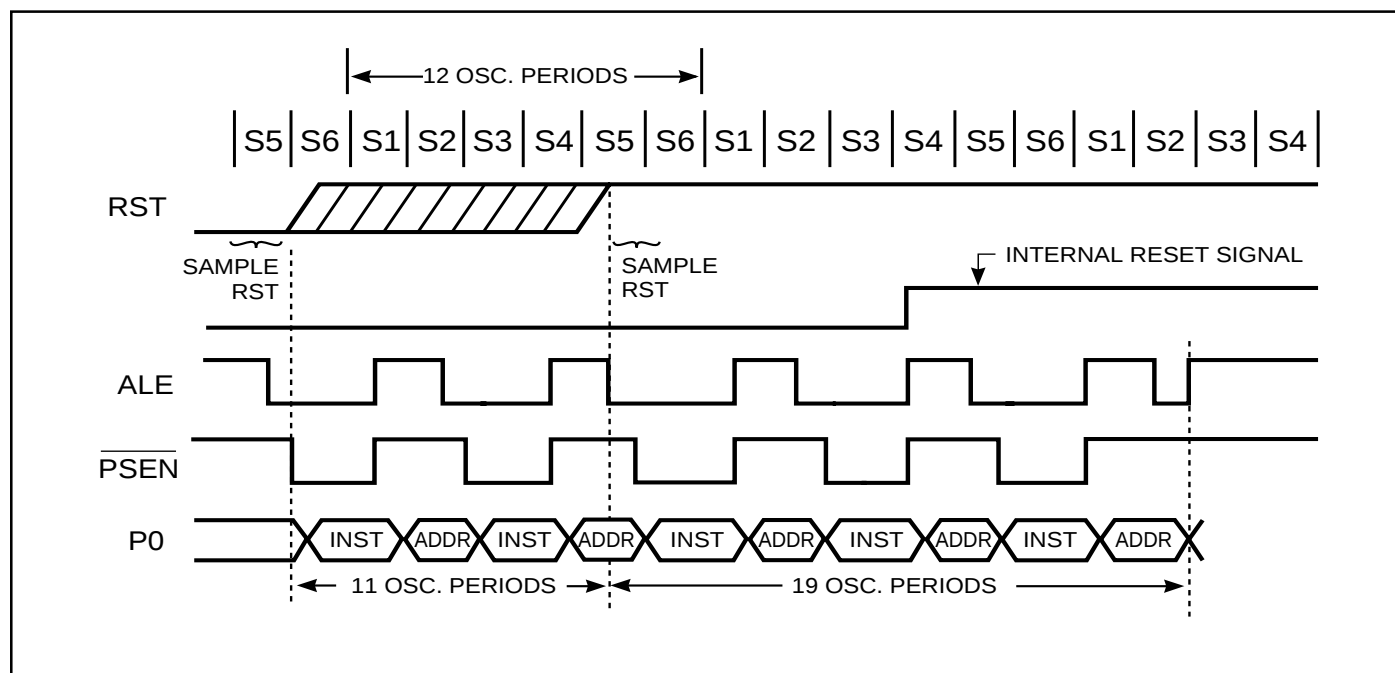
Figure 18. Reset Timing
