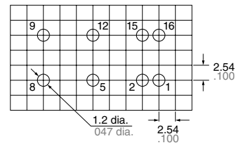
PC board pattern (Copper-side view) DSP1a-PS, DSP1a-PSL2
