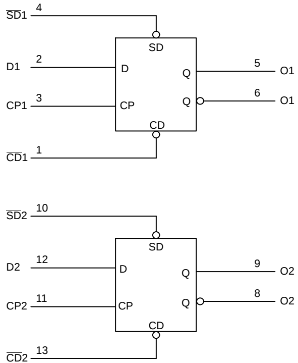
Figure 2. Logic Diagram
