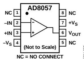
Figure 2. R-8 (SOIC)
