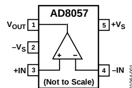
Figure 1. RT-5 (SOT-23)
