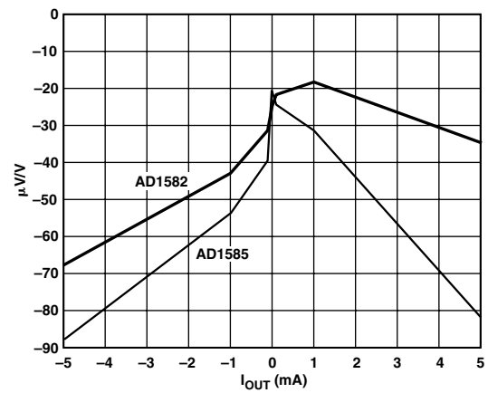
TPC 5. Line Regulation vs. I_{LOAD}
