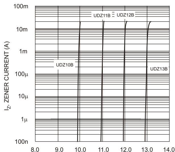
V_Z , ZENER BREAKDOWN VOLTAGE (V) Fig. 4 Typical Reverse Characteristics, UDZ10B - UDZ13B
