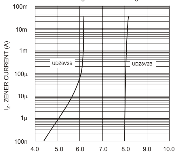
V_Z , ZENER BREAKDOWN VOLTAGE (V) Fig. 3 Typical Reverse Characteristics, UDZ6V2B - UDZ8V2B
