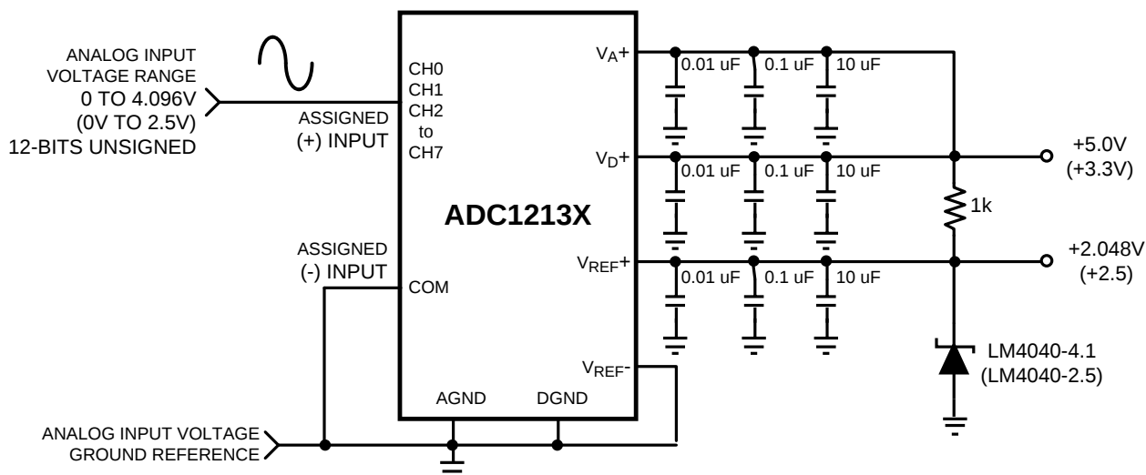
Figure 69. Single-Ended Biasing
