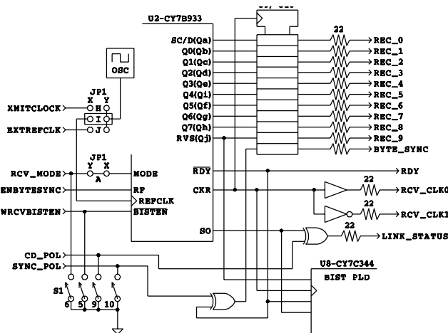
Figure 13. HOTLink Receiver Parallel Interface
