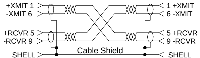
Figure 27. STP Cable Connectors
