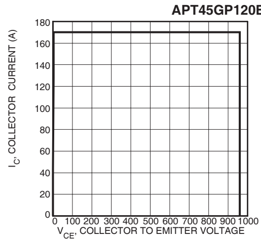
Figure 18, Minimum Reverse Bias Safe Operating Area
