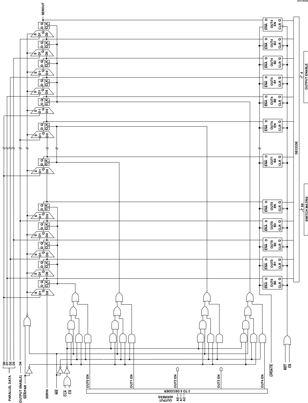
Figure 7. Logic Diagram
