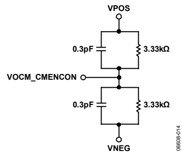
Figure 14. VOCM_CMENCON Input (Also See ESD Protection Map, Figure 19)
