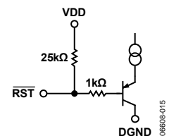
Figure 15. \overline{\text{RST}} Input (Also See ESD Protection Map, Figure 19)
