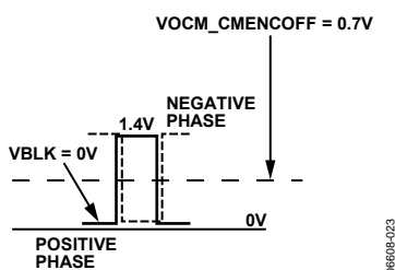
Figure 48. Output at the AD8178 Pins for 0 V to 0.7 V Input Differential Pulse, V_{BLK} = 0\text{ V} , V_{OCM\_CMENCOFF} = 0.7\text{ V}
