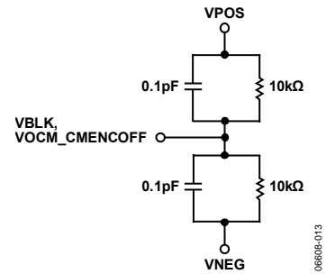
Figure 13. VBLK and VOCM_CMENCOFF Inputs (Also See ESD Protection Map, Figure 19)
