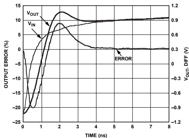
Figure 25. Settling Time
