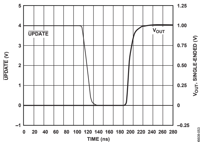
Figure 44. Enable Time
