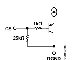
Figure 17. \overline{\text{CS}} Input (Also See ESD Protection Map, Figure 19)
