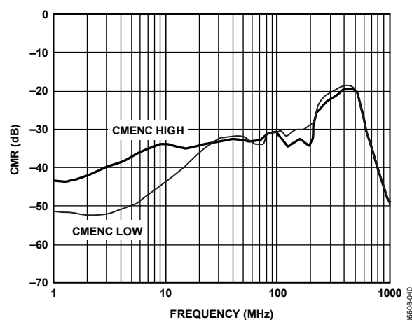
Figure 31. Common-Mode Rejection
