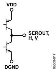
Figure 18. SEROUT, H, V Logic Outputs (Also See ESD Protection Map, Figure 19)
