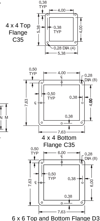
6 x 6 Top and Bottom Flange D35
