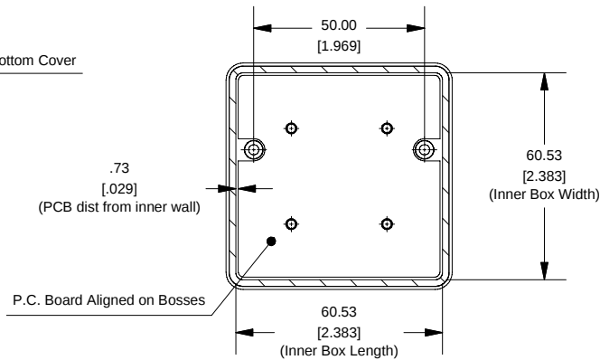
SECTION B-B (Inside of Bottom Cover)
