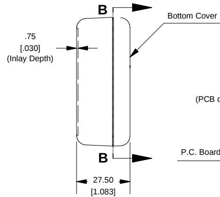
End View of Assembly
