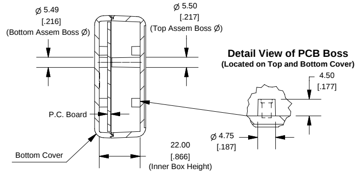
SECTION B-B (Inside of Bottom Cover)
