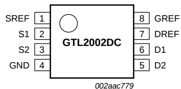
Fig 4. Pin configuration for VSSOP8
