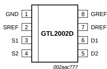
Fig 2. Pin configuration for SO8
