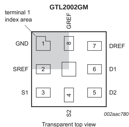
Fig 5. Pin configuration for XQFN8
