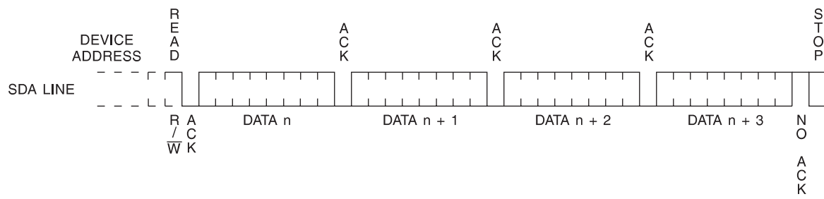
Figure 6. Sequential Read
