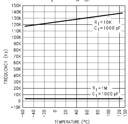
VHC4046 VCO OUT vs Temperature V_{CC} = 4.5V R_2 = \text{OPEN} V_{COIN} = V_{CC}/2
