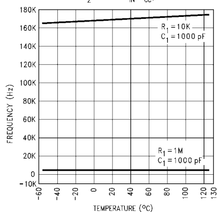
VHC4046 VCO OUT vs Temperature V_{CC} = 6V R_2 = \text{OPEN} V_{COIN} = V_{CC}/2
