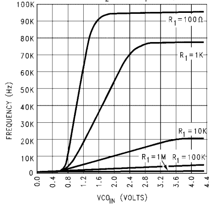
VHC4046 V_{COIN} vs f_{OUT} V_{CC}=4.5\text{V}
