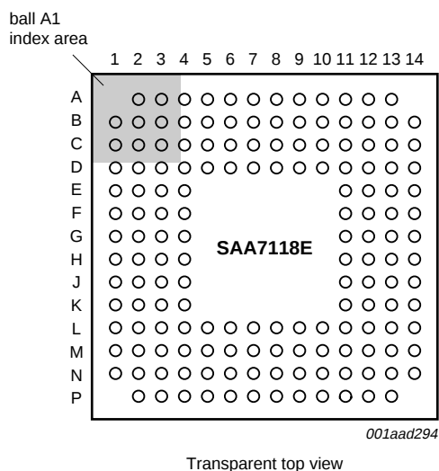
Fig 3. Pin configuration (LPGA156)
