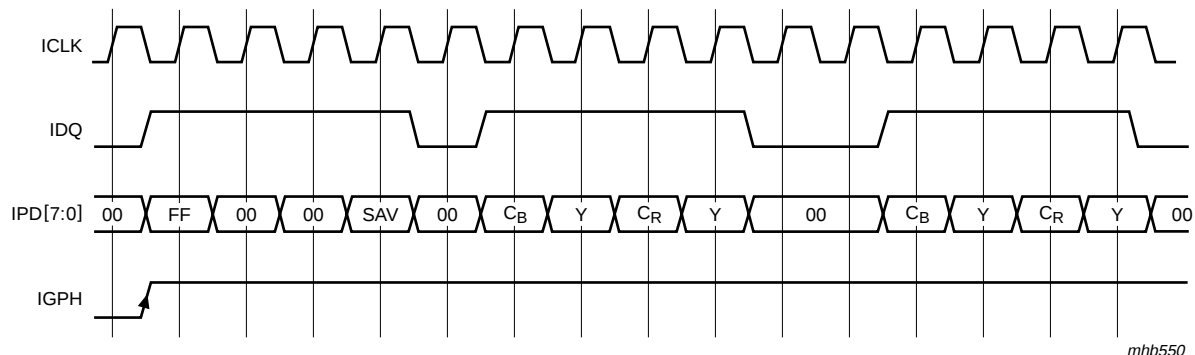
Fig 42. Output timing I port for serial 8-bit data at start of a line (ICODE = 1)
