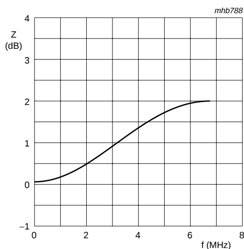
Fig 27. C_B-C_R low-pass filter frequency response
