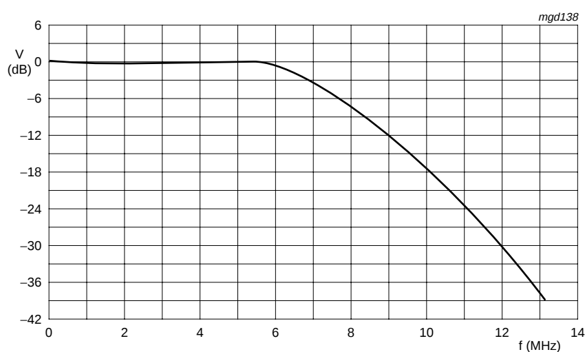
Fig 4. Anti-alias filter
