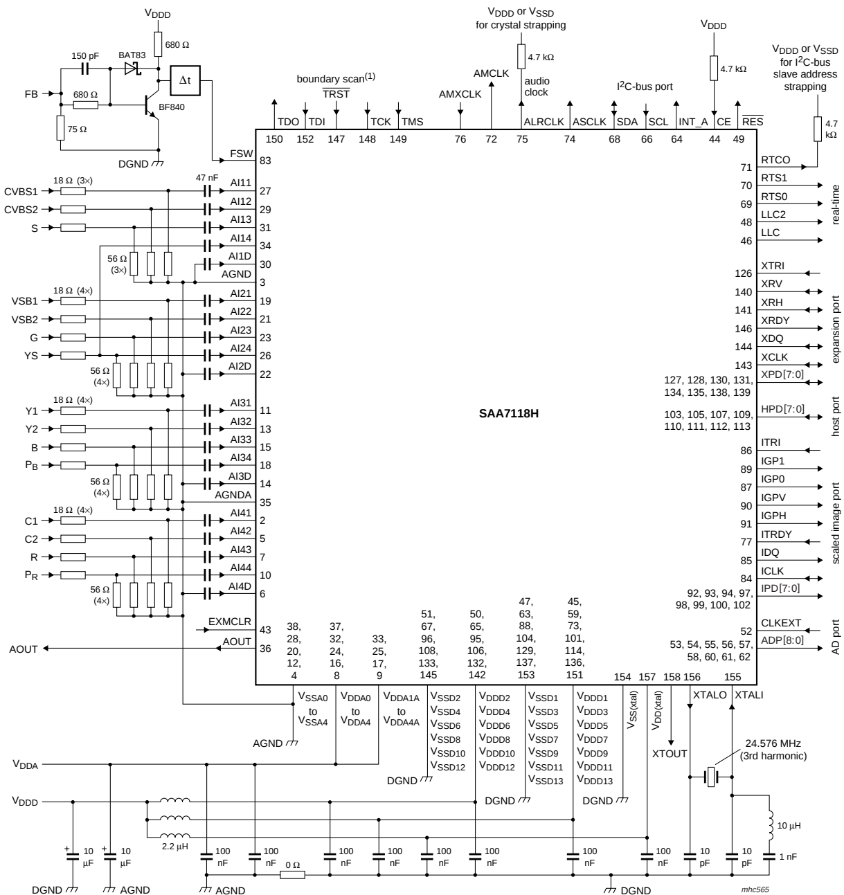
Fig 93. Application example with 24.576 MHz crystal (QFP160 package)
