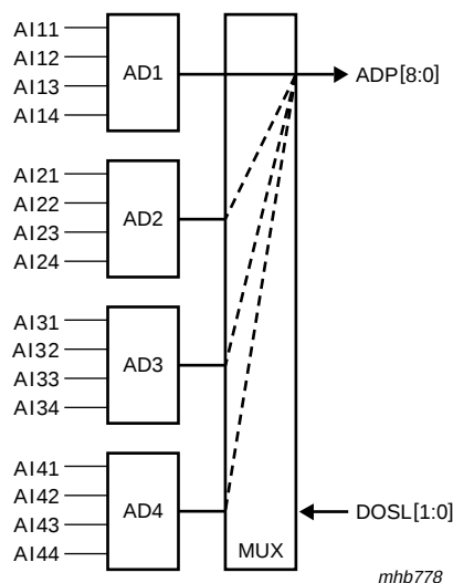
Fig 90. VSB modes (use CVBS modes with REFA = 1, DOSL = 0 to 3 and GAFIX = 1)
