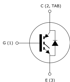
TO-247
